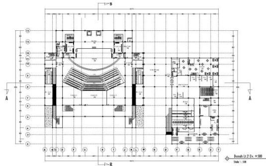
Gambar 12. Denah Lantai Elevasi +500
